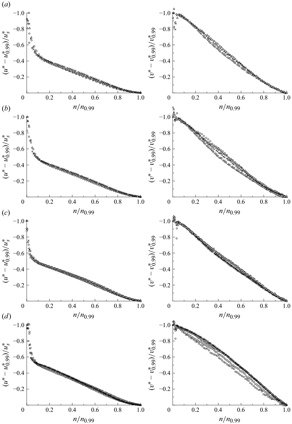
Figure 11. The dissimilar scaling of the mean velocity components at locations s/c = 0.10 ( \square ), s/c = 0.20 ( \circ ), s/c = 0.30 ( \triangle ), s/c = 0.40 ( \times ) and s/c = 0.50 ( * ) for four controlled cases: (a) \alpha = 12.5^\circ and C_\mu = 1.25 \times 10^{-3} , (b) \alpha = 12.5^\circ and C_\mu = 0.25 \times 10^{-3} , (c) \alpha = 15.0^\circ and C_\mu = 1.25 \times 10^{-3} , (d) \alpha = 15.0^\circ and C_\mu = 0.25 \times 10^{-3} .
