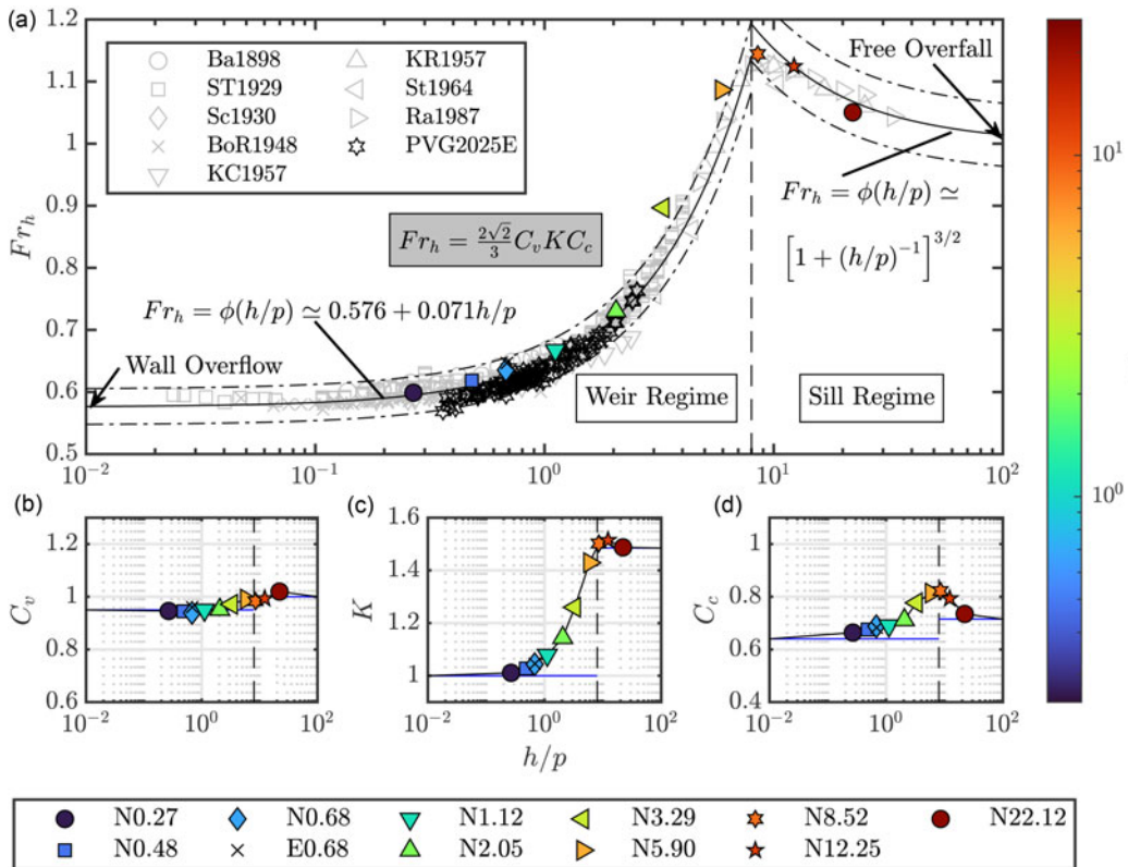
Figure 4. (a) Fr_h versus h/p for the entire weir-sill range, with the historical data (table 1) plotted. Classical empirical equations relating h/p and Fr_h are also shown by a solid line, after Kandaswamy and Rouse (1957), with dash-dotted lines representing \pm 5\% variation. For all data, Re_h > 3.5 \times 10^4 . For cases shown in table 2: (b) C_v versus h/p ; (c) K versus h/p ; and (d) C_c versus h/p . Approximate values of C_v , K and C_c for the upper and lower limits of h/p , representing the respective cases of the free overfall and wall overflow, are given by blue horizontal lines.
