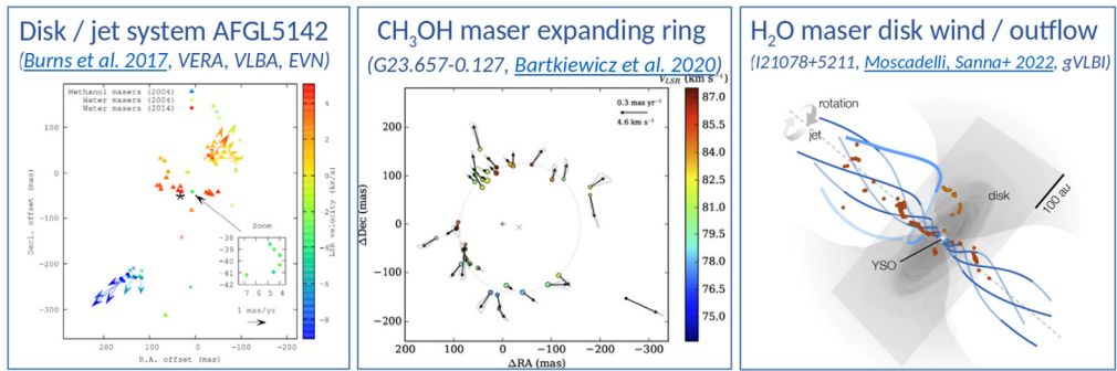
Figure 1. Three examples of kinematic structures traced by VLBI observations of masers around young massive protostars from Burns et al. (2017), Bartkiewicz et al. (2020), and Moscadelli et al. (2022).
