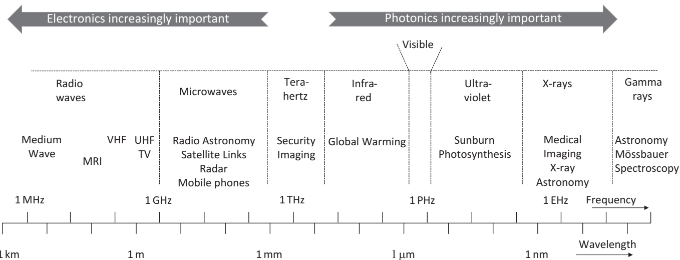
Figure 1.1 The principal regions of the electromagnetic spectrum. The boundaries between the various regions are fuzzy (except for the tiny visible part), though most regions have a presence in everyday life.
